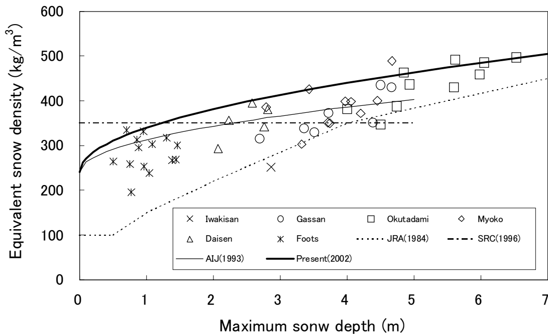
Figure 2: Equivalent snow density, \rho_2 vs maximum snow depth, H_{\max}
