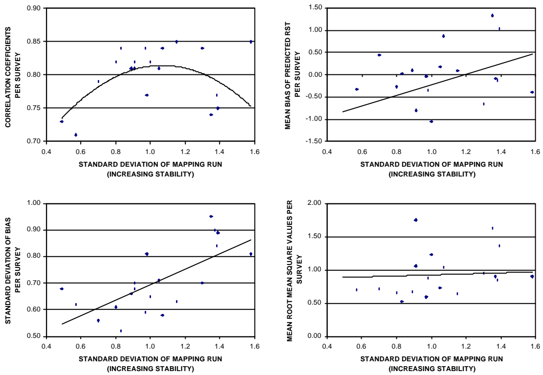
Figure 1 Model performance quantified in correlation coefficients, bias, standard deviation of bias and RMS at different levels of atmospheric stability.
