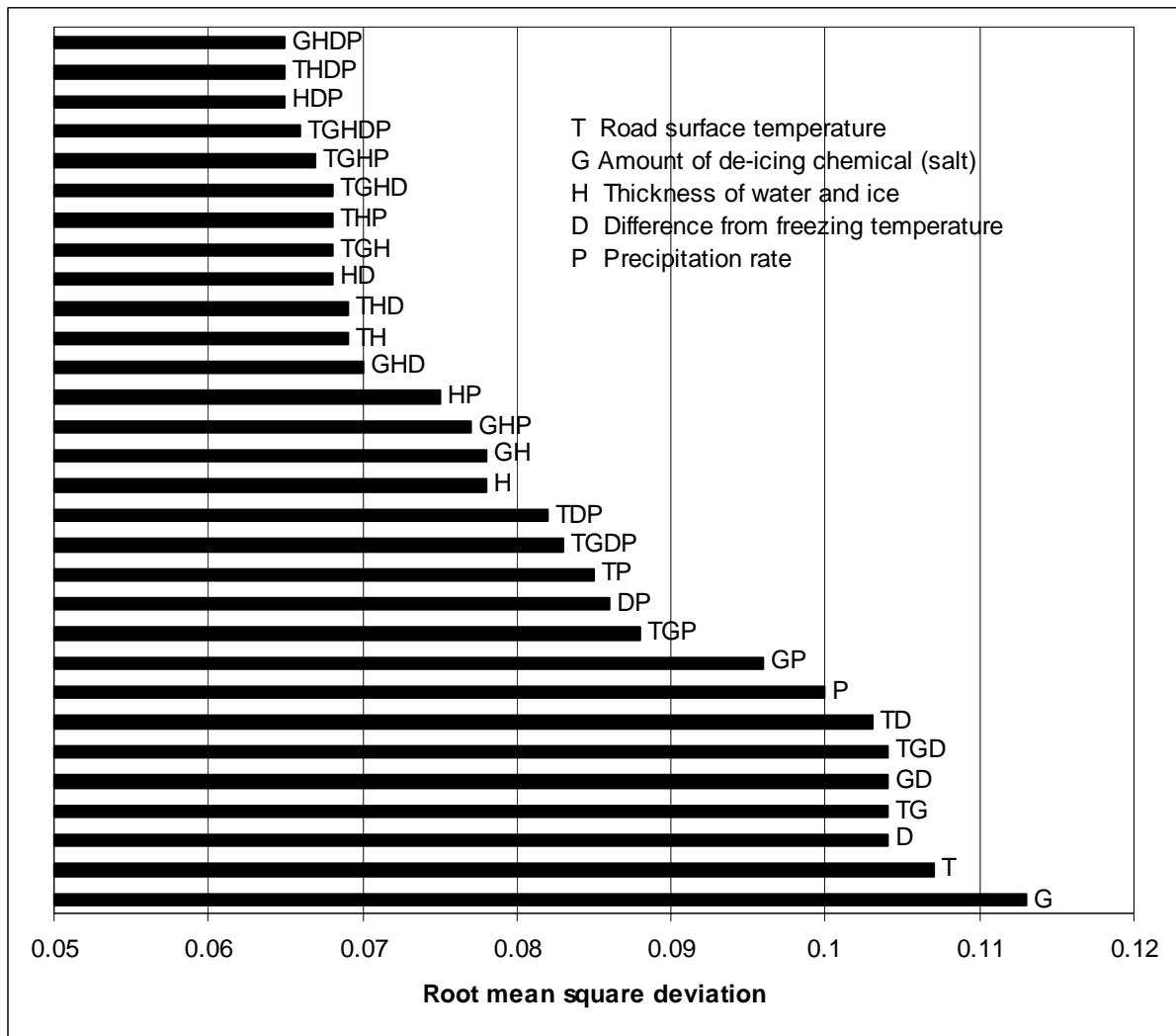
Figure 3 The root mean square deviation of the trained artificial neural network with different inputs. The letters (TGHDP) indicate the combinations of the input data used.
