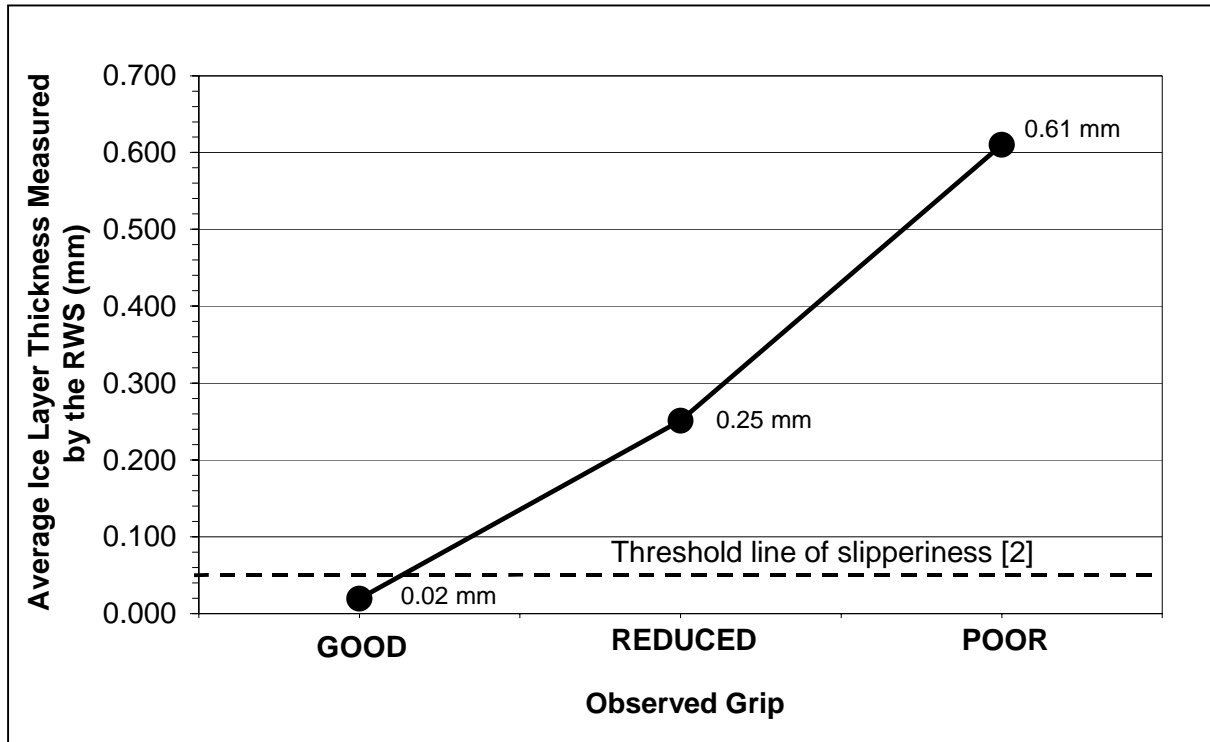
Figure 2 The average thickness of the ice layer compared to the grip observations. It is determined in laboratory tests [2] that the ice layer of 0.05 mm is the threshold value for dangerously slippery roads.
