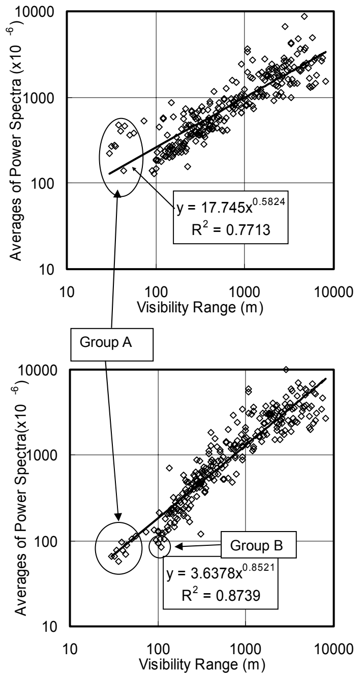
Figure 7 Averages of power spectra versus visibility range (number of data: 270)
