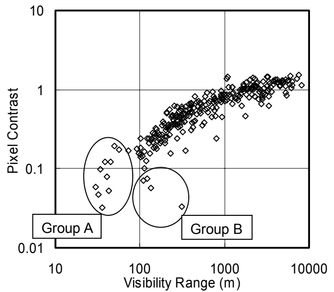
Figure 4 Pixel contrast versus visibility range in the daytime (number of data: 270 ).
