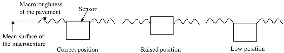
Figure 4 : Positioning of a sensor in the pavement
