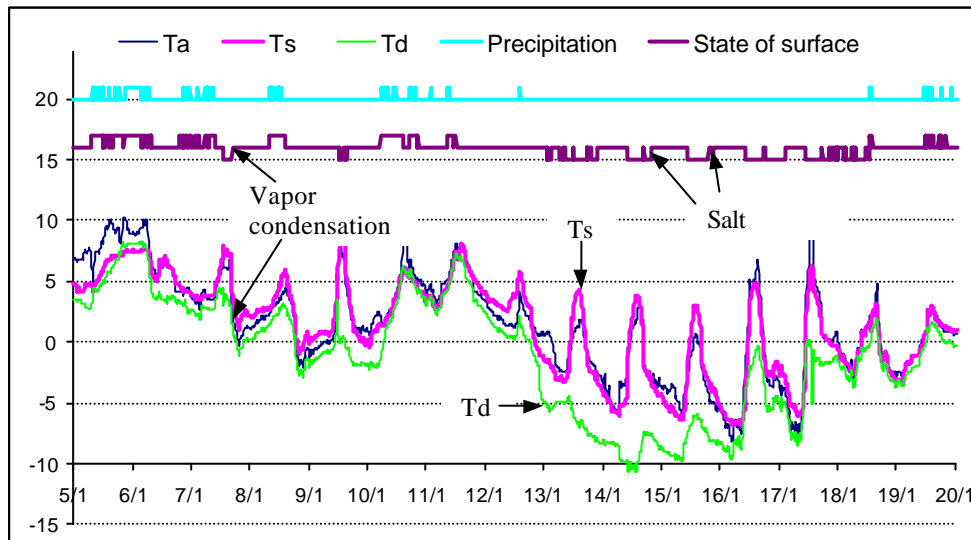
Figure 2 : Graphical representation of the RWIS measurements made on January 2001 for station S02.
