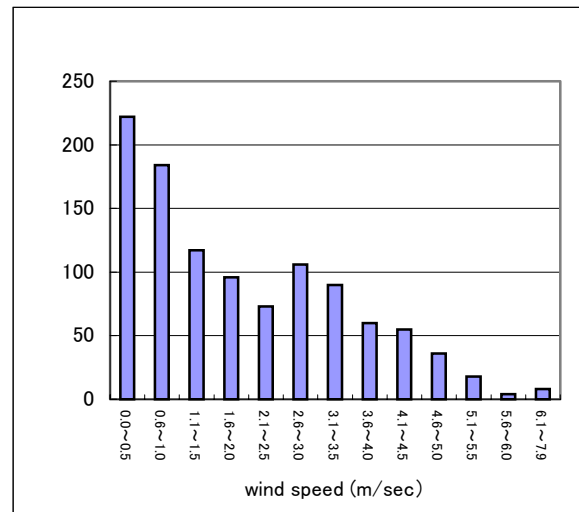
Fig. 6 Wind speed occurrence frequency at Point A
