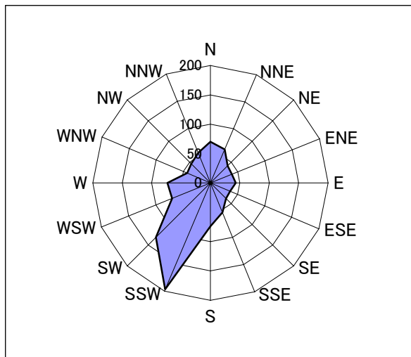
Fig. 5 Wind direction occurrence frequency at Point A
