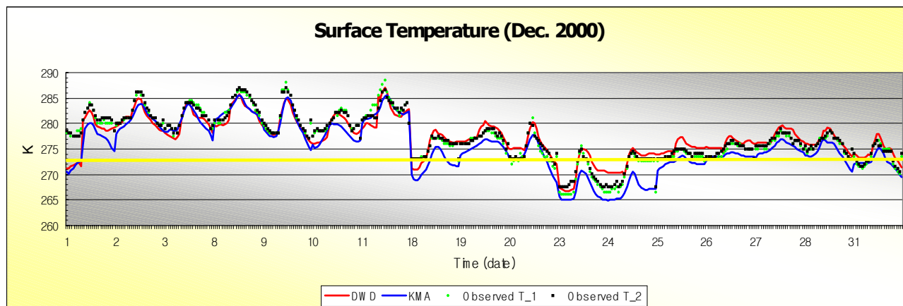
Figure 1. Calculated road surface temperature by using the both model and Observed data
