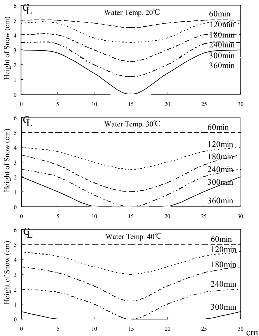
Fig. 5 Influence of water temperature to the snow melting process (Type.3)
